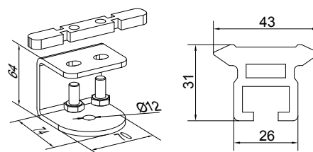
Rail support
