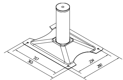
Absorber post
