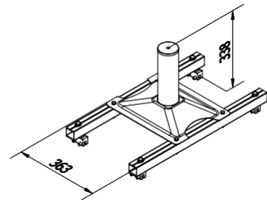
Absorber post
